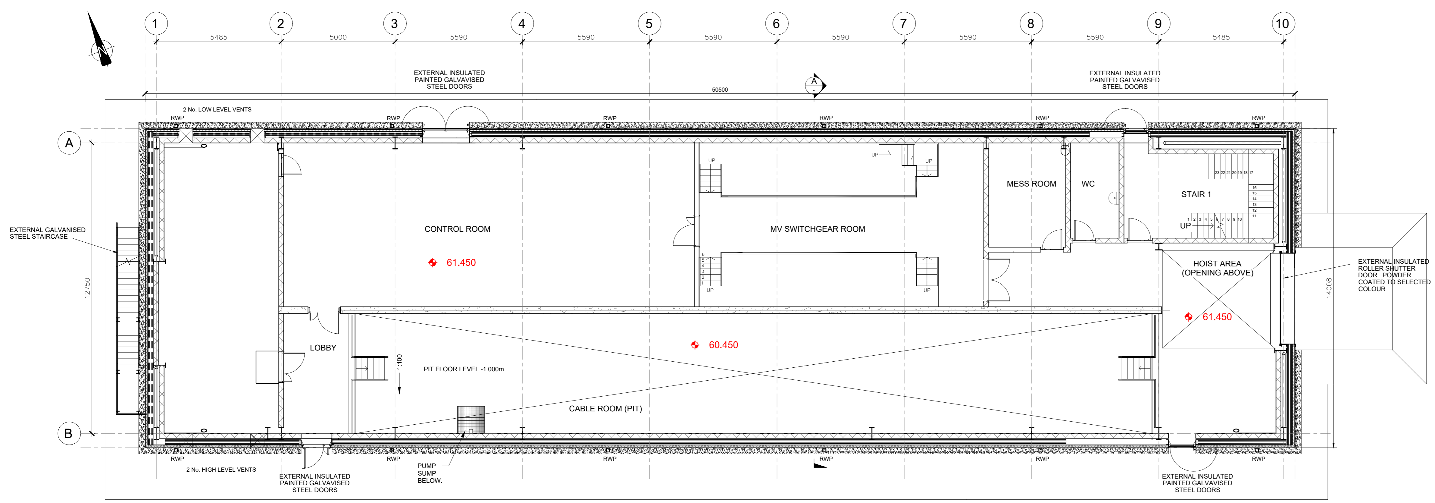
GROUND FLOOR PLAN SCALE 1:100
