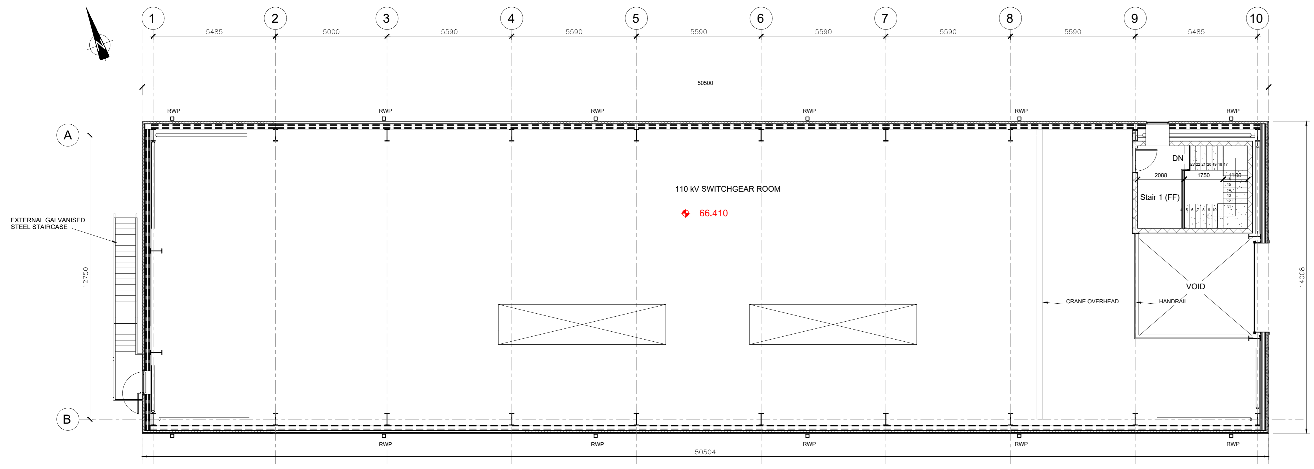
FIRST FLOOR PLAN SCALE 1:100
